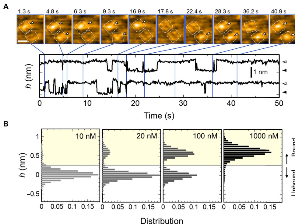
Fig. 2. HS-AFM captured AgTx2 binding to the channel with single-molecule resolution. (A) Time-lapse images of AgTx2 binding to and dissociation from the KcsA channels (top; see also movie S1) and time courses of the averaged height h (nm) around the center of the extracellular surface (0.8 nm by 0.8 nm area) of two corresponding K^+ channels (bottom). White dotted squares represent regions of interest for visualization of the tetrameric channels. Spontaneous AgTx2 bindings on the channels (bottom). The bathing electrolyte solution contains 10 mM Hepes (pH 7.5) and 100 mM KCl. The scale bar in the first AFM image represents 5 nm. (B) Height histograms at 10, 20, 100, and 1000 nM AgTx2. The height of the extracellular surface of the AgTx2-unbound channel was set to 0 nm. Height transitions used in the histograms were measured in 10 mM Hepes (pH 7.5) containing 200 mM KCl. The number of data frames used for the histograms were 8604, 250,846, 33,701 and 35,453 for 10, 20, 100, and 1000 nM AgTx2, respectively.
