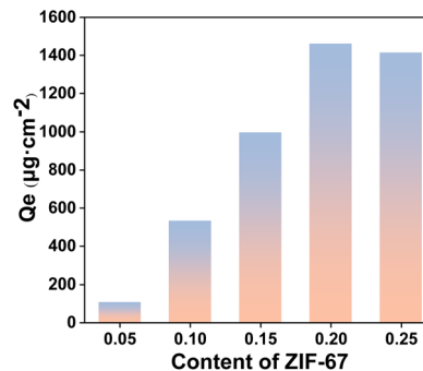
Fig. 6 The addition of ZIF-67 in ZIF-67/PVDF ( T = 298.15 K, \text{pH} = 6-8 , C_0 (CIP) = 400 \text{mg L}^{-1} , the area of the membrane = 4 \text{cm}^2 , t = 15 h).
