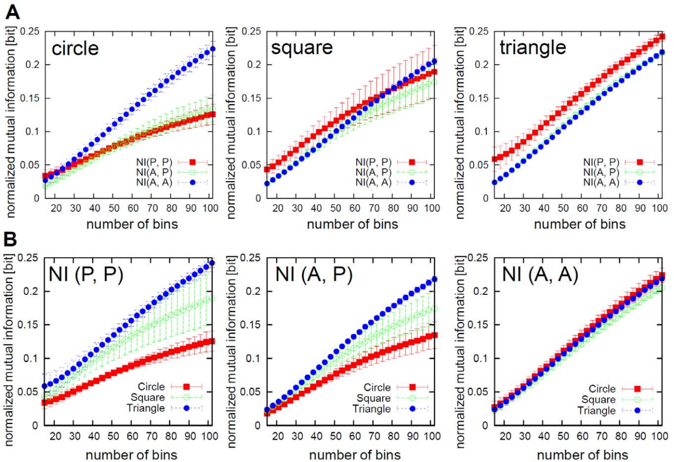
Figure 12. Comparisons of normalized mutual information according to the number of bins. A. Comparisons of normalized mutual information ( NI(P,P) , NI(A,P) and NI(A,A) ) according to the number of bins in the circular (left), square (middle), and triangular (right) cases. B. Comparisons of the circular, square and triangular cases for NI(P,P) , NI(A,P) and NI(A,A) . The same plots of A. are rearranged. doi:10.1371/journal.pone.0037805.g012
