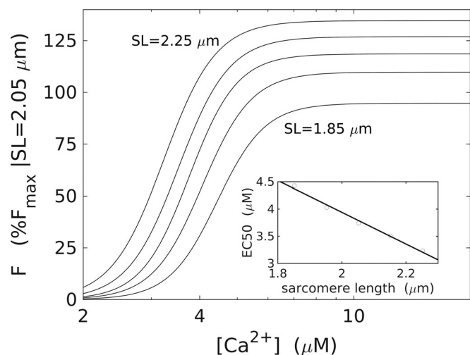
Figure 5. Dependence of the calcium sensitivity on sarcomere length. (a) Hill-type F-pCa for sarcomere lengths (SLs) = 1.85, 1.95, 2.05, 2.15, and 2.25 \mu\text{m} . Forces are normalized to the maximum force measured at SL = 2.05 \mu\text{m} . The data do not show a change in the Hill coefficient. (b) Increase in the Ca^{2+} sensitivity (decreasing [Ca^{2+}] at half-maximum) with increasing SL, measured from the position of the inflection point in the fitted Hill curves from panel a. Adapted from Dobesh et al. (2002).
