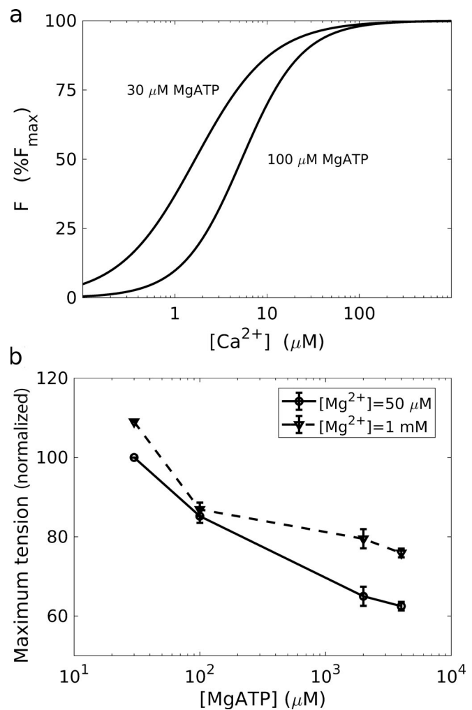
Figure 6. Dependence of the force–calcium relationship on MgATP in the rat heart. (a) Decrease in Ca 2+ sensitivity (increase in [Ca 2+ ] at half-maximum) as [MgATP] increases from 30 to 100 \mu\text{M} ( [Mg^{2+}] = 50 \mu\text{M} ). (b) Decrease in the maximum tension with increasing [MgATP]. Adapted from Best et al. (1977).
