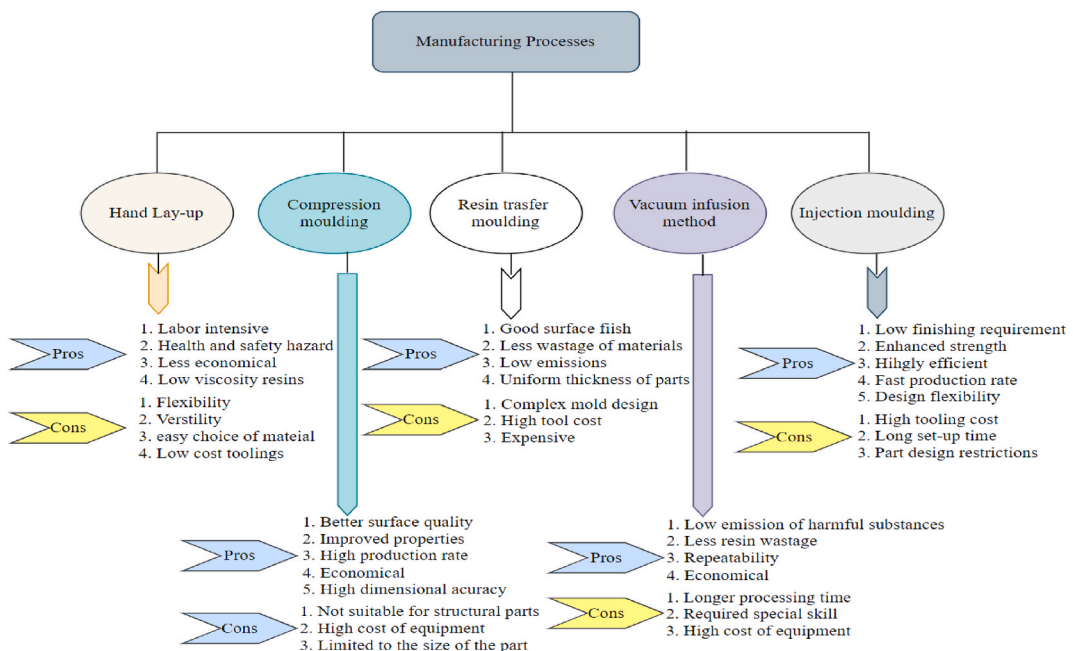
Fig. 4. Common manufacturing processes for natural fiber-based composites.
