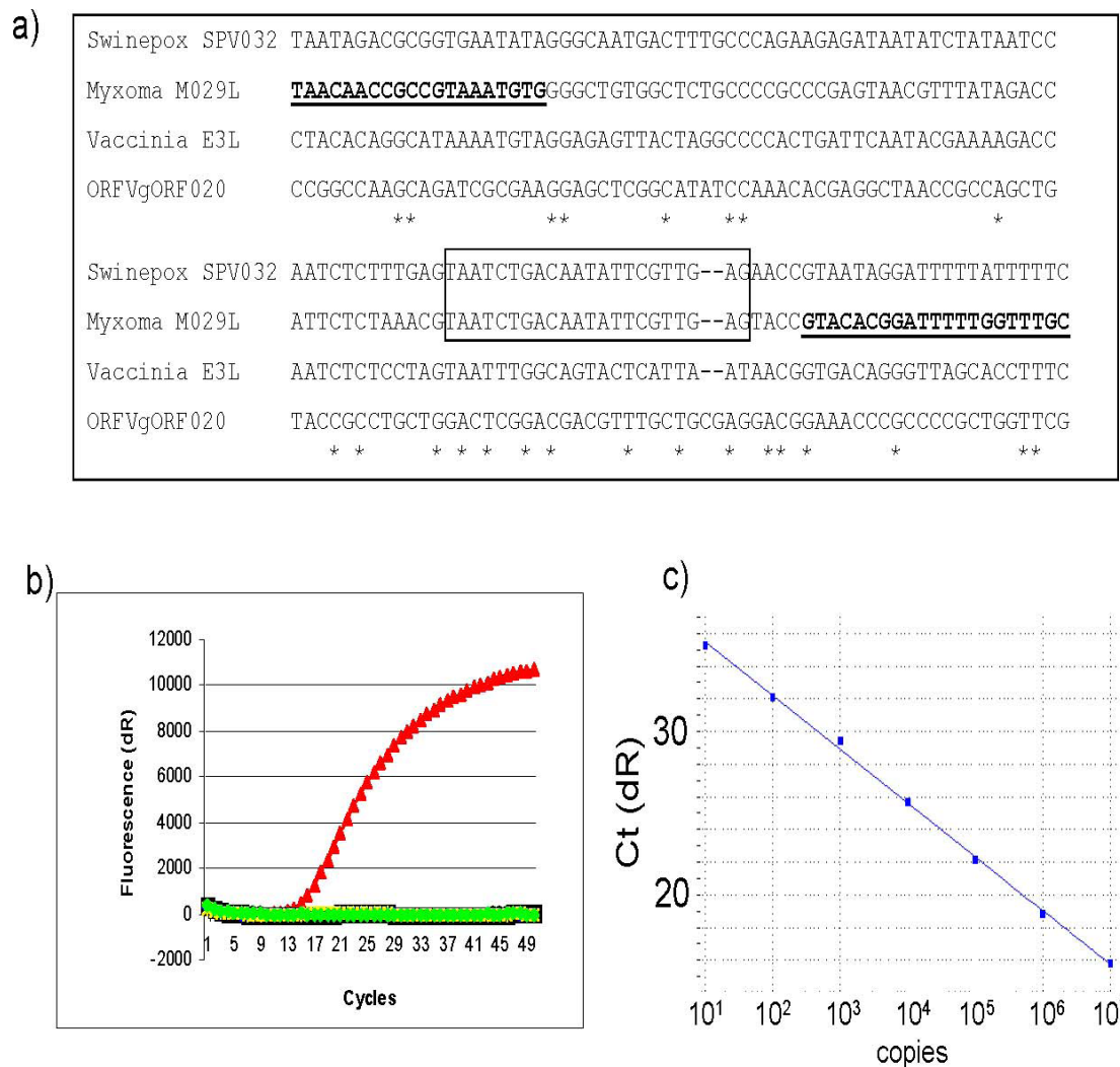
Figure 1 Design and properties of myxoma virus specific qPCR assay. Panel (a). The sequence of the myxoma virus M029L gene [GenBank: NC_001132] was aligned with the homologous E3L genes from vaccinia virus (WR strain, [GenBank:AY243312], swinepox [GenBank:NC_003389] and Orf virus [GenBank:NC_005336]) using ClustalW2. The positions of the myxoma virus specific primers (myxE3Lfor and myxE3Lrev) (in bold type and underlined) and the MGB-probe (within the rectangle) which recognizes a sequence that is identical in myxoma virus and swinepox virus are indicated. Panel (b). Viral DNA was prepared from cell culture grown samples of vaccinia virus (WR strain, blue diamond), myxoma virus (red triangle), swinepox virus (black square) and Orf virus (black circle) and each was assayed (in parallel and with negative (water) controls (yellow and green symbols)) in the qPCR assay for myxoma virus as described in Materials and Methods. Panel (c) Serial 10-fold dilutions of a plasmid, including the myxoma M029L gene, containing between 10^1 and 10^7 copies were tested in the myxoma virus assay. The gradient of the line is -3.293 and the efficiency of the PCR reaction was calculated as 101.2%.
