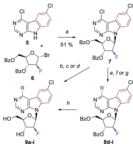
Scheme 1 Reagents and conditions: a) KOH, TDA-1, MeCN, r.t., 30 min, then Br-arabinose 6 in MeCN, r.t., 20 h; b) aq. NH 3 , dioxane, 100 °C, 2 days; c) 1 M NaOMe in MeOH, MeOH, r.t., 3 h; d) NaSMc, EtOH, r.t., 4 h; e) (Me) 3 Al (2 M in toluene), Pd(PPh 3 ) 4 , THF, 70 °C, 18 h; f) R-B(OH) 2 , K 2 CO 3 , Pd(PPh 3 ) 4 , toluene, 100 °C, 17–36 h; g) R-SnBu 3 , PdCl 2 (PPh 3 ) 2 , DMF, 100 °C, 17–18 h; h) 1 M NaOMe in MeOH, MeOH, r.t., 2–18 h.
