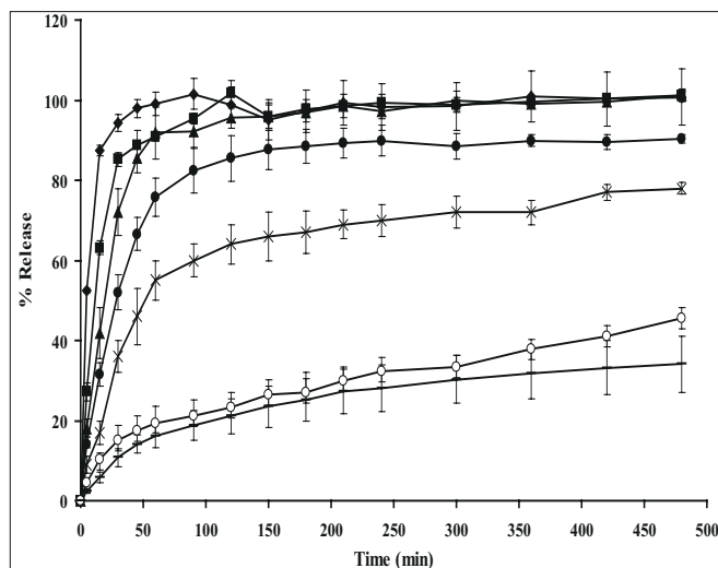
Fig. 1: Drug release profiles of indomethacin formulations Drug release profiles of indomethacin from tablets containing (—◆—) 0% HPMC; (—■—) 5% HPMC; (—▲—) 10% HPMC; (—●—) 15% HPMC; (—×—) 20% HPMC; (—○—) 25% HPMC and (—) capsules in phosphate buffer pH 6.2 (n=3).
