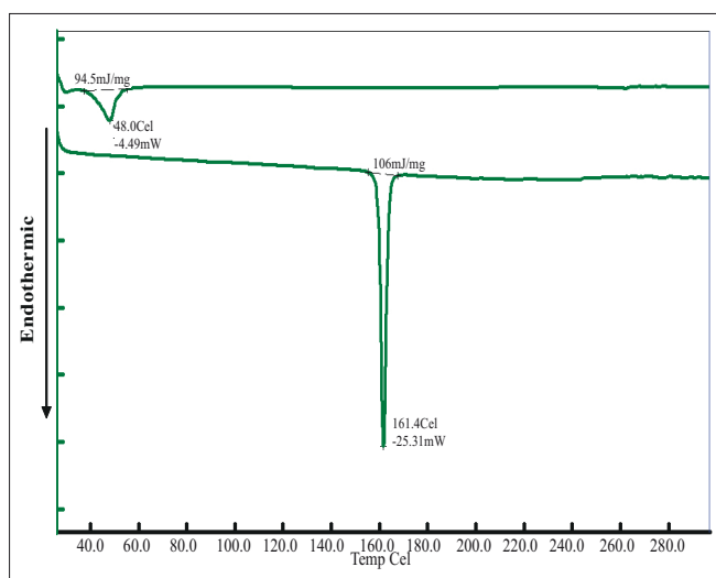
Fig. 4: DSC thermograms of PEG 4000 and PEG 400 mixture and indomethacin.
