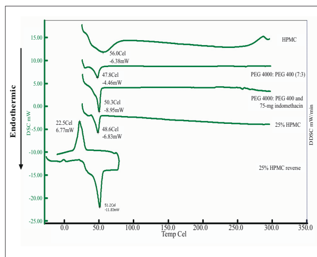
Fig. 5: DSC thermograms of HPMC and indomethacin tablets.
