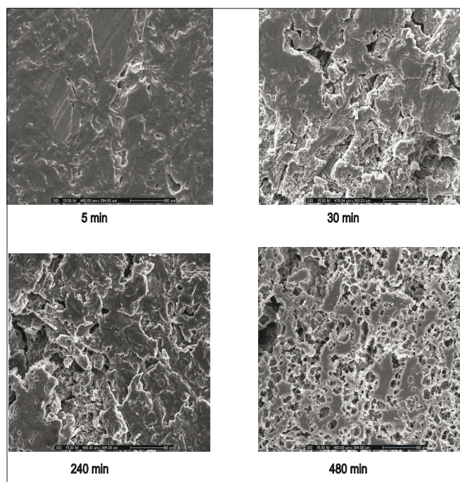
Fig. 7: SEM micrographs of tablets of 75 mg indomethacin. Scanning electron microscope micrographs of tablets containing 75 mg indomethacin and 25% HPMC in 70:30 PEG 4000:PEG 400 system after dissolution test in phosphate buffer pH 6.2 at different time interval with magnification of 250X.
