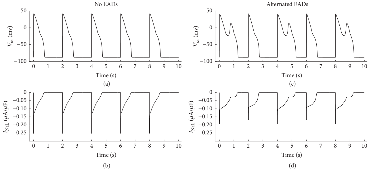
FIGURE 1: (a) No EAD was produced when CaMKII phosphorylation level was in control ( CaMK_0 = 0.05 ). (b) Corresponding I_{NaL} when no EADs occurred in (a). (c) Alternated EADs were produced when I_{NaL} phosphorylation by CaMKII was enhanced with CaMK_0 of 0.12 and other targets' phosphorylation levels were in control ( CaMK_0 = 0.05 ). (d) Corresponding I_{NaL} when alternated EADs occurred in (c). Under these conditions, CL was 2000 ms and I_{Kr} was blocked by 85%.
