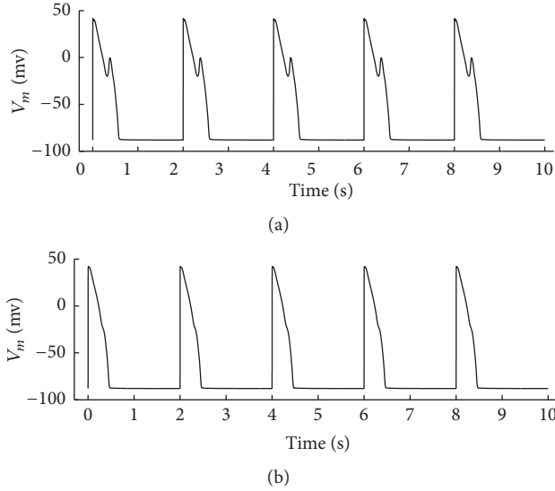
FIGURE 2: (a) EADs were induced when 1 \mu\text{M} ISO was applied and I_{K_r} was blocked by 85%. In (b), EADs disappeared when I_{K_r} blockage was reduced to 77%. Cycle length was set 2000 ms and CaMKII phosphorylation level to all targets was kept control ( \text{CaMK}_0 = 0.05 ).
