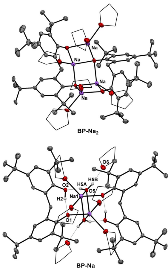
Figure 2. Molecular structures of sodium bisphenolate complexes.
