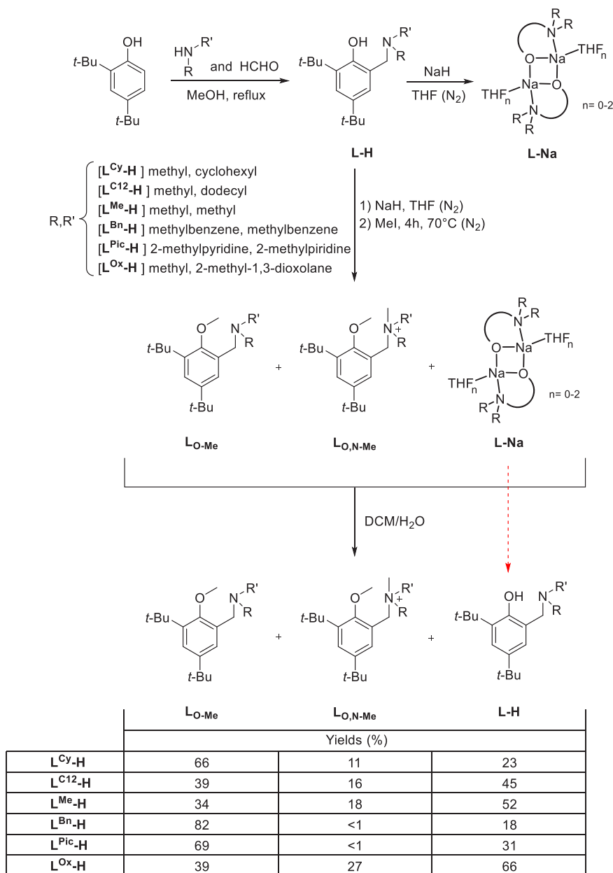
Scheme 3. General Synthesis to Obtain Methylated Aminophenols
