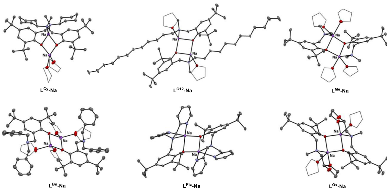
Figure 1. Molecular structures of sodium aminophenolate complexes.
