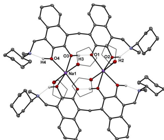
Figure 3. Molecular structure of sodium complex BN Cy -Na.
