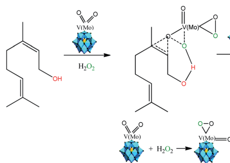
Scheme 6 Propose of reaction pathway of vanadium-doped sodium phosphomolybdate salt-catalyzed nerol epoxidation reaction with hydrogen peroxide (adapted from ref. 15, 17 and 38).
