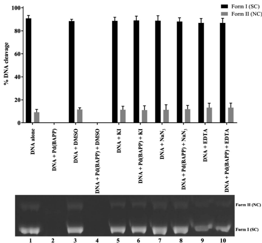
Fig. 10 Cleavage of pBR322 plasmid DNA ( \sim 0.4 \mu\text{g} ) by the ROS scavengers (0.2 M) (DMSO, KI, \text{NaN}_3 ) in the presence and absence of the complex (100 \mu\text{M} ) in Tris-HCl/NaCl buffer (pH = 7.2) at 37 ^\circ\text{C} for 1.5 h.
