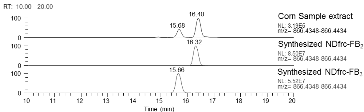
Figure 5. Chromatograms of NDfrc-FB 2 and NDfrc-FB 3 in corn powder extract in comparison with the chemically synthesized species (scan event 1).
