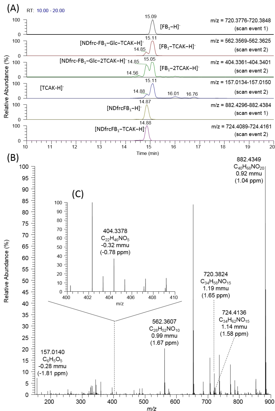
Figure 2. Detection and identification of \text{NDfrc-FB}_1 . Mass chromatogram with scan results (scan events 1 and 2) (A); full mass spectrum obtained at 14.87 min (scan event 1) (B); and mass range magnification of full mass spectrum ( m/z : 400–410) obtained at 14.87 min (scan event 1) (C).
