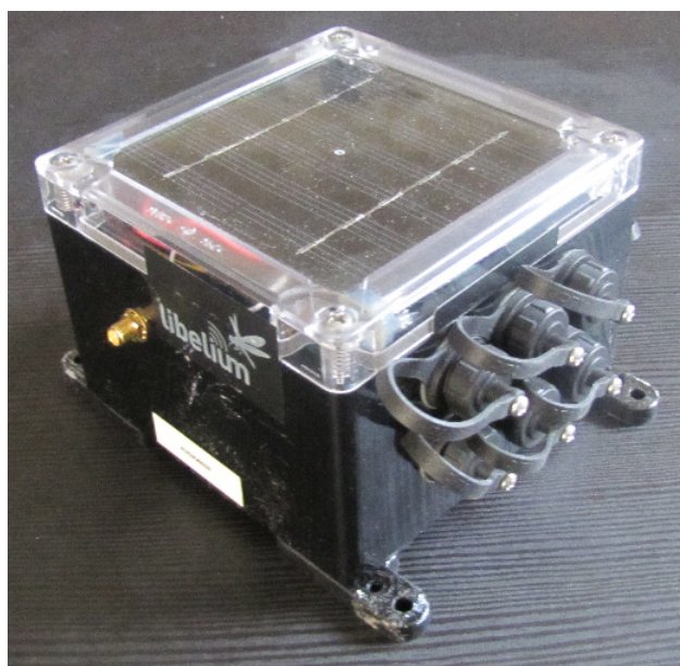
Figure 2. Wasmote Plug & Sense platform.
