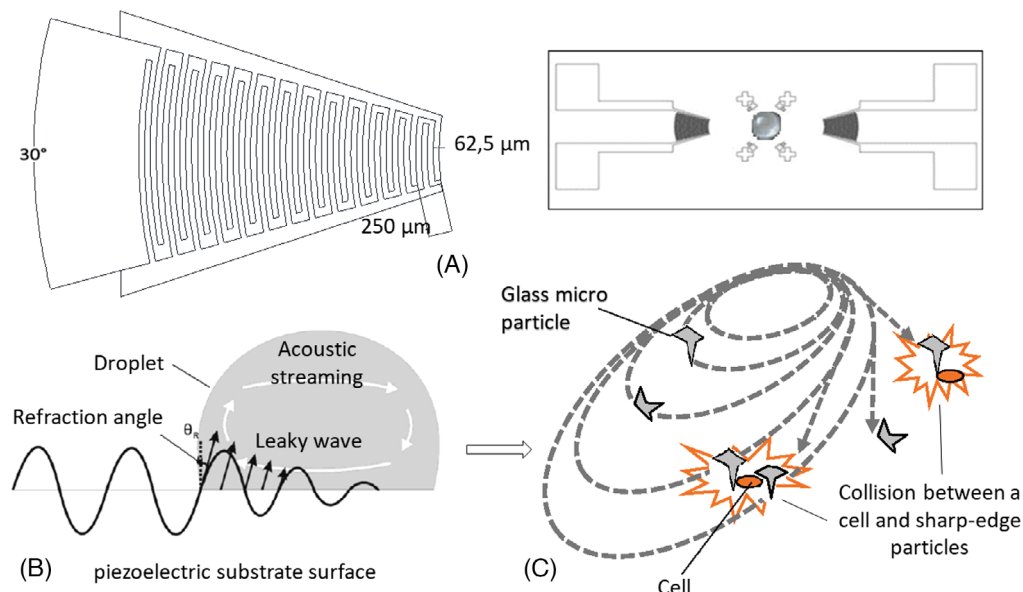
FIGURE 2 Cell lysis principle of surface acoustic wave-based approach using sharp-edge irregulated micro-glass particles: (A) Schematic of focused IDT and device design. (B) The longitudinal wave causes acoustic streams within the droplet, creating a non-contact motion in a radial direction at high speed. (C) Collision between cells and sharp-edge glass micro particles inside the droplet causing cell lysis.
