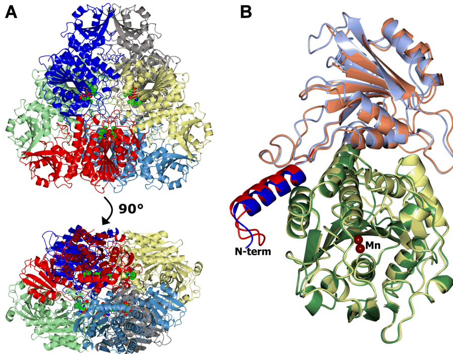
FIG 1 Structures of the LAP-As. Protein chains are shown in a ribbon representation. (A) Hexamer of the TbLAP-A --bestatin complex colored by chain. The six bestatin ligands and associated metals are shown as spheres and lie on the inside of the hexamer. (B) Superposition of TbLAP-A and LmLAP-A protomers. The TbLAP-A N-terminal helix ( \alpha 1 ) is blue, the N-terminal domain is light blue, and the C-terminal domain is green. For LmLAP-A , \alpha 1 is red, the N-terminal domain is coral, and the C-terminal domain is lemon. The Mn^{2+} ions in the active sites are shown as tan spheres. This and subsequent structure images were made in CCP4mg (63), and superpositions were carried out with SSM (64).
