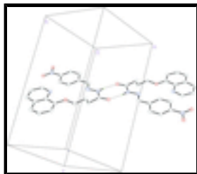
Fig. 2. The cyclic hydrogen-bonded dimer with hydrogen bonds shown as dashed lines. H atoms, except for those involved in hydrogen bonds, are not included.
