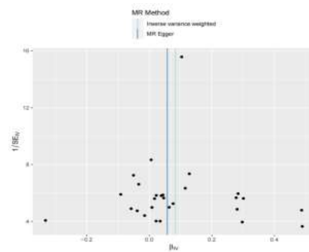
Funnel plot
