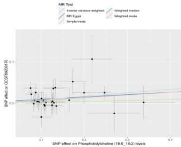
Scatter plot
