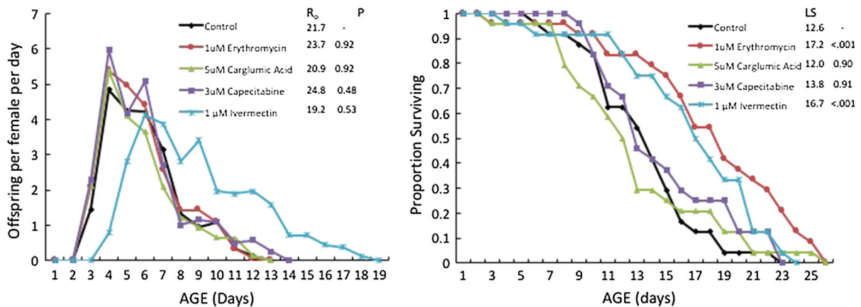
Fig. 3 Reproductive life table with 24 rotifers per treatment of 4 drugs binding to aging pathway proteins. R_0 net fecundity of females over their reproductive lifetimes, P probability of significant difference from control by one-way ANOVA and
