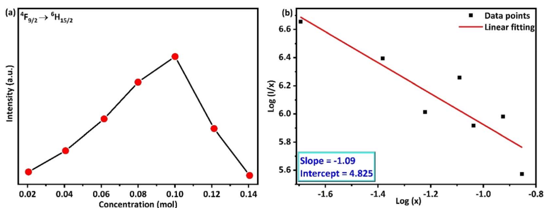
Fig. 9 (a) Variation of emission intensity ( {}^4\text{F}_{9/2} \rightarrow {}^6\text{H}_{15/2} ) with variation in the doping concentration (b) logarithmic variation of the PL intensity of \text{Dy}^{3+} doped \text{BaLa}_2\text{ZnO}_5 phosphor.
