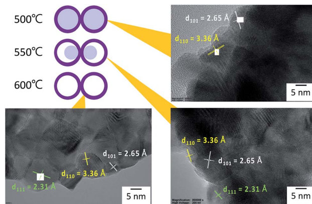
Fig. 4 High magnification TEM images of heat-treated samples at 500 °C, 550 °C, and 600 °C.
