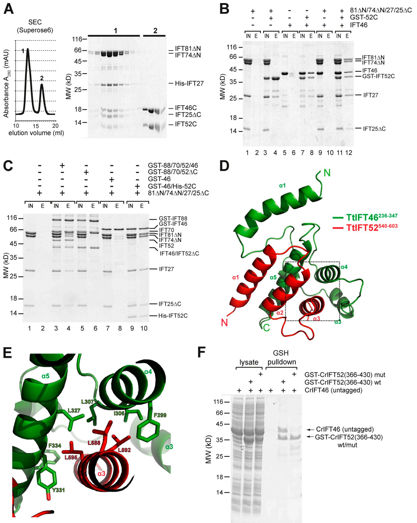
Figure 4. Structural and biochemical analysis of the IFT52C/46C complex. (A) SEC analysis showing that a dimeric IFT52C/46C complex can form a stable complex with IFT81 \Delta N/74 \Delta N/27/25 \Delta C. The IFT81 \Delta N/74 \Delta N/27/25 \Delta C tetramer was incubated with an excess of IFT52 382-454 /46 165-319 (IFT52C/46C), and the resulting products were analyzed by SEC using a Superose 6 column. The chromatogram and the SDS-PAGE analysis of the peak fractions show that stoichiometric levels of the IFT52C/46C are shifted from the low-molecular weight peak 2 to the high molecular weight peak 1. (B) GST
