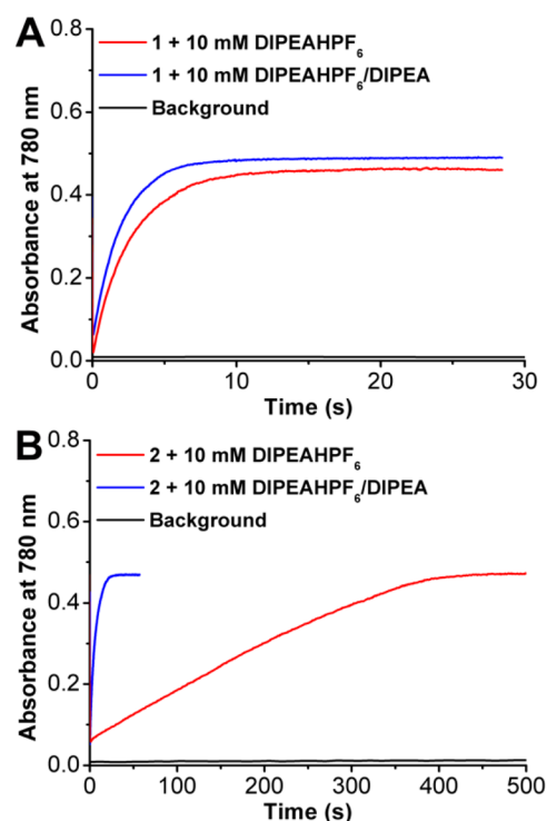
Fig. 4 Change in absorbance at 780 nm over time as a result of the formation of [Cp* 2 Fe] + by ORR catalyzed by Mn( P- tbu dmbpy)Cl 1 (A) with DIPEAHPF 6 (red) and DIPEAHPF 6 /DIPEA (blue) and Mn( nPr dmbpy)Cl 2 (B) with DIPEAHPF 6 (red) and DIPEAHPF 6 /DIPEA (blue). Black: buffered control. Conditions: 40 μM [Mn], 4.05 mM [O 2 ], 1 mM [Cp* 2 Fe], 10 mM [DIPEAHPF 6 /DIPEA]; control: 4.05 mM O 2 , 1 mM Cp* 2 Fe, 12.5 mM DIPEAHPF 6 /DIPEA.
