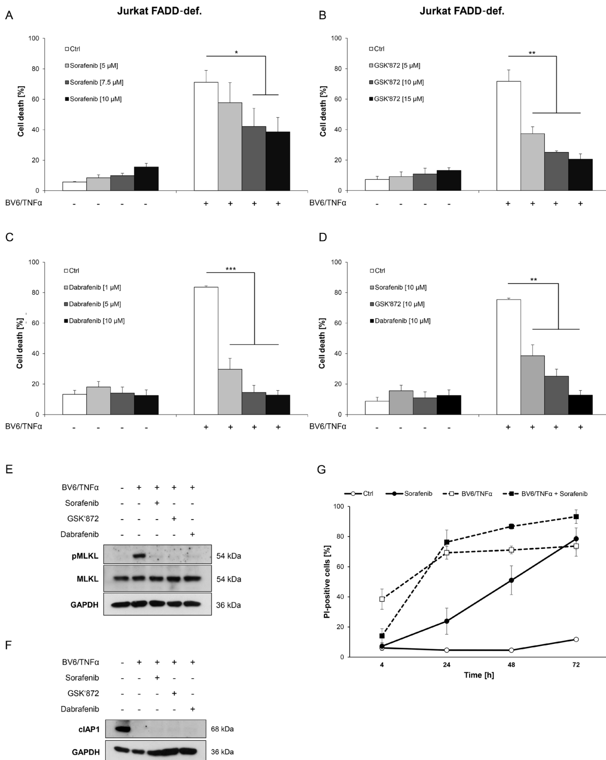
Figure 3: Sorafenib protects ALL cells from BV6/TNF \alpha -induced necroptosis. (A–C) FADD-deficient Jurkat cells were treated for 4 hours with 1 \mu M BV6 and 1 ng/ml TNF \alpha in the presence or absence of indicated concentrations of Sorafenib (A), GSK'872 (B) or Dabrafenib (C). (D) FADD-deficient Jurkat cells were treated for 4 hours with 1 \mu M BV6 and 1 ng/ml TNF \alpha in the presence or absence of 10 \mu M Sorafenib, 10 \mu M GSK'872 or 10 \mu M Dabrafenib. (E and F) FADD-deficient Jurkat cells were treated for 2 hours with 1 \mu M BV6 and 1 ng/ml TNF \alpha in the presence or absence of 10 \mu M Sorafenib, 6 \mu M GSK'872 or 0.6 \mu M Dabrafenib. Expression levels of MLKL, phospho-MLKL and cIAP1 were analyzed by Western blotting, expression of GAPDH served as loading control. (G) FADD-deficient Jurkat cells were treated with or without 1 \mu M BV6 and 1 ng/ml TNF \alpha in the presence or absence of 10 \mu M Sorafenib for the indicated time points. Cell death was determined by FSC/SSC analysis (A–D) or PI staining (G) and flow cytometry. Mean and SD of at least three experiments performed in triplicate are shown; * P < 0.05; ** P < 0.01; *** P < 0.001.
