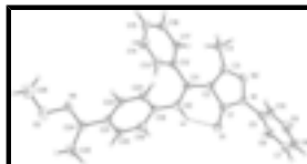
Fig. 1. The molecular structure of the title compound with atom numbering scheme. Displacement ellipsoids for non-hydrogen atoms are drawn at the 30% probability level. Intramolecular hydrogen bond is shown as a dashed line.
