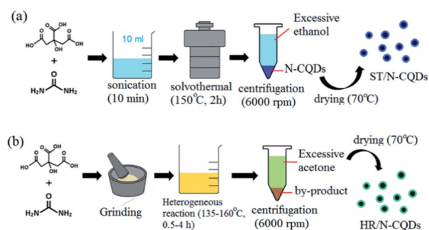
Fig. 1 Synthetic procedures for (a) ST and (b) HR.
