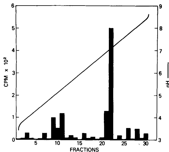
FIG. 1. Isoelectric focusing of ^{125}\text{I} -labeled human LP. 1% Ampholine (pH 3-10) and 4.5% acrylamide. Gel lengths were 2.5 \times 10 mm. Constant voltage, 200 V, was applied for 18 h at 4^\circ\text{C} . Gels were cut every 2 mm and radioactivity and pH were measured on each fraction.
