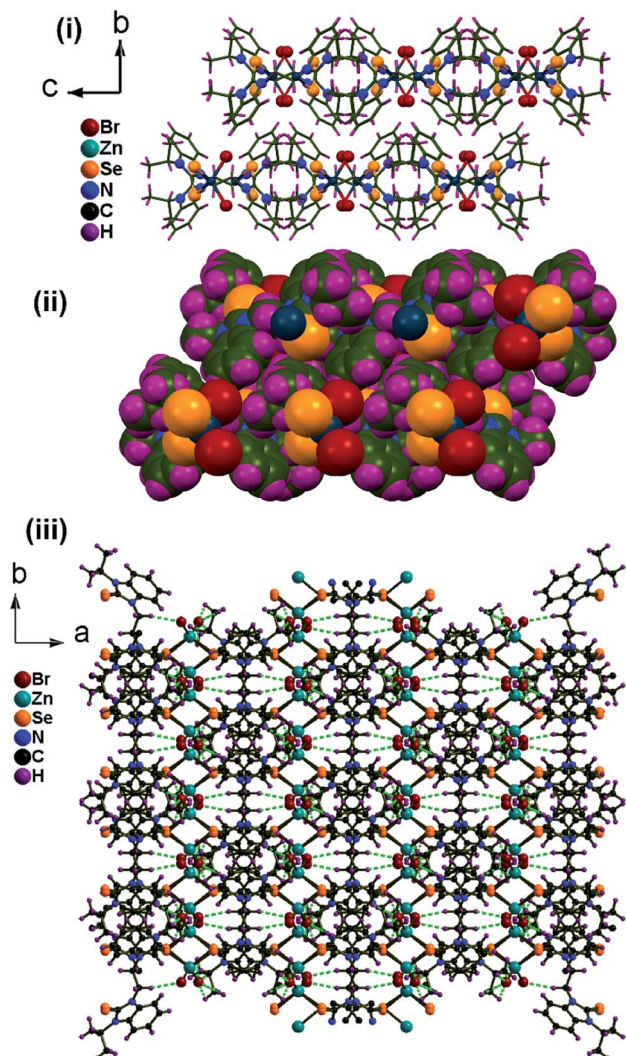
Fig. 3 (i) Arrangements of one-dimensional coordination polymers in 1 (view along a axis). (ii) Space-filling model of one-dimensional coordination polymers in 1 (view along a axis). (iii) Perspective view of the sheet structure of 1 through hydrogen bonding (view along the c axis).
