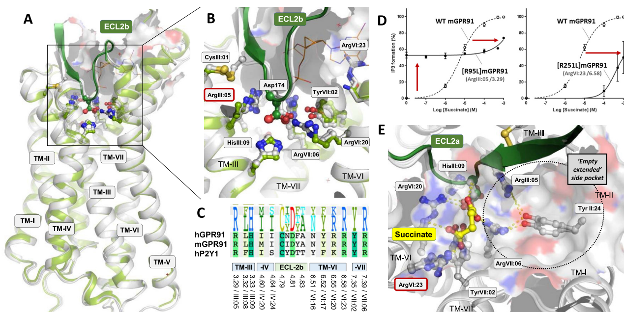
Figure 2: Molecular modeling of the GPR91-succinate complex. A ) Comparison of the of P2Y1 X-ray structure (pdbid:4xnw, green) and the homology of the human and mouse GPR91 receptors (gray) generated based on the P2Y1 structure with ECL-2b buried deep in between TM-III, -V and -VII highlighted in dark green. Side view from TM-IV and -V. B ) Detailed side view (with TM-IV and -V removed) of the interactions between ECL-2b – in particular Asp174 – and transmembrane residues in the P2Y1 receptor and the corresponding interactions in the models of hGPR91 and mGPR91. C ) 'Pseudo-sequence' of conserved network of polar and positively charged residues, which are found close to Asp174 (ECL-2b) in the main ligand binding pocket of P2Y1, and h and mGPR91. Positions are annotated both with Ballesteros Weinstein and Schwartz numbering (used in most figures). D ) Dose-response curves for succinate in HEK-293 cells transfected with either the WT mGPR91 (dotted line) or the [R95L]mGPR91 (Arg:05/3.29) (left panel) proposed to affect activity as shown in panel B or [R251L]mGPR91 (ArgVI:23/6.58) (right panel) which is proposed to affect activity directly through interaction with succinate binding panel E. Red arrows indicate shifts in potency and efficacy induced by mutations (N = 3). E ) Extracellular view of the top-ranking binding conformation of succinate (yellow) in complex with hGPR91. Note interaction of one carboxylate of succinate with the backbone -NH of Asp174 in ECL-2b and with ArgVII:06 (from the 'bottom' of the pocket) and the other carboxylate with ArgVI:23. The unoccupied pocket extending towards TM-I and -II from the proposed binding site of succinate, which we in the following try to exploit for binding of synthetic succinate analogs is indicated by a dotted circle.
