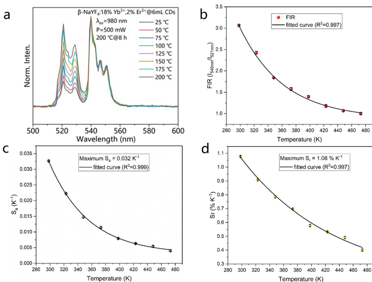
Fig. 6 (a) The normalized UC emission spectra as a function of temperature for the \beta\text{-NYF@6CDs} composite; (b–d) the parameters of FIR, S_a , and S_r as functions of temperature.
