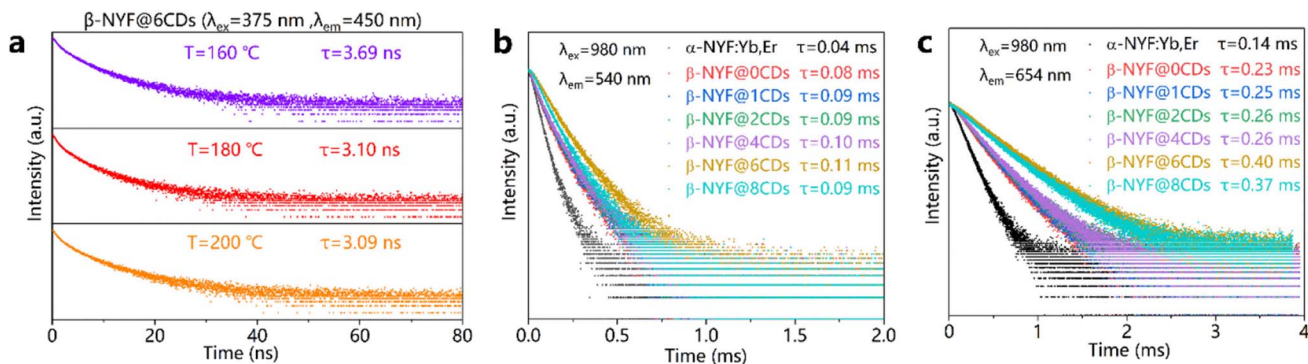
Fig. 5 (a) Luminescence decay curves of the \beta -NYF@6CDs composite at different reaction temperatures; luminescence decay curves of (b) green and (c) red emissions for \beta -NaYF 4 :18%Yb 3+ ,2%Er 3+ @CDs composites with varying content of CDs.
