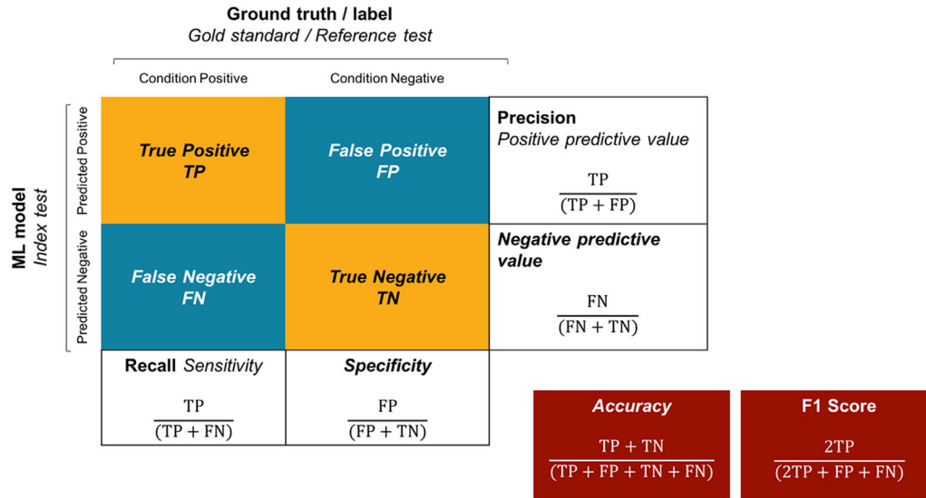
Figure 2. Overview of confusion matrix/contingency table. Differences in nomenclature for machine learning (boldface type) and classical statistics (italic type) and where overlapping (boldface and italic) are highlighted.
