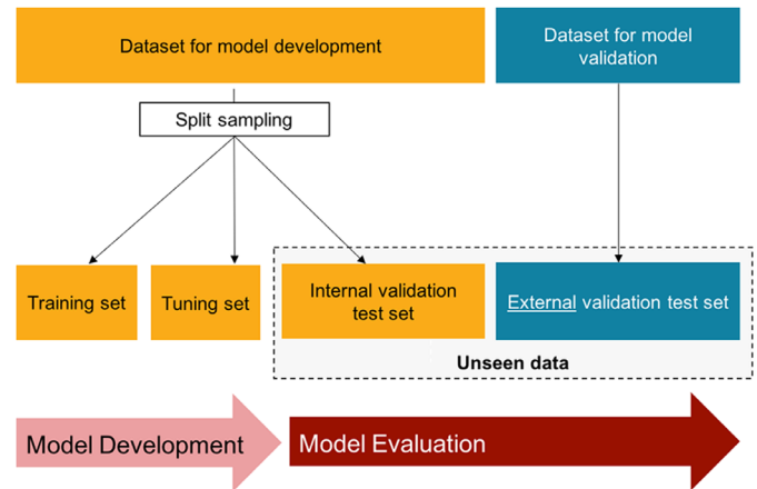
Figure 1. Overview of datasets involved in a machine learning diagnostic algorithm: model development and evaluation.
