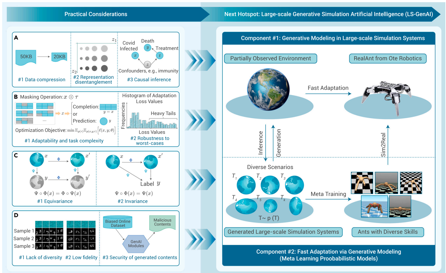
Figure 1. Practical considerations and the roadmap of LS-GenAI The left supports the utilities of LS-GenAI, while the right is the roadmap to achieve via the doubly generative paradigm.
