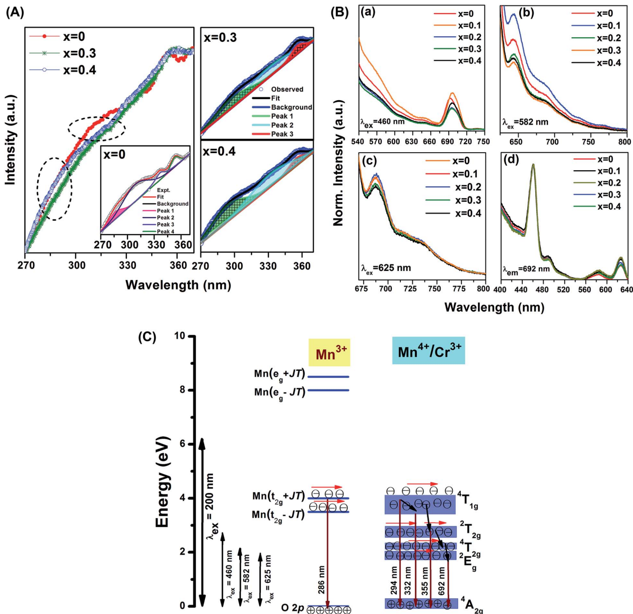
Fig. 3 (A) The emission spectra of \text{GdMn}_{1-x}\text{Cr}_x\text{O}_3 ( x = 0, 0.3 and 0.4 ) under the excitation wavelength of 200 \text{ nm} (Inset depicts the deconvoluted peaks). (B) The emission spectra of \text{GdMn}_{1-x}\text{Cr}_x\text{O}_3 ( x = 0, 0.1, 0.2, 0.3 and 0.4 ) at (a) \lambda_{\text{ex}} = 460 \text{ nm} , (b) \lambda_{\text{ex}} = 582 \text{ nm} , (c) \lambda_{\text{ex}} = 625 \text{ nm} and (d) the excitation spectra after monitoring \lambda_{\text{em}} = 692 \text{ nm} . (C) The proposed energy band diagram for Cr doped \text{GdMnO}_3 .
