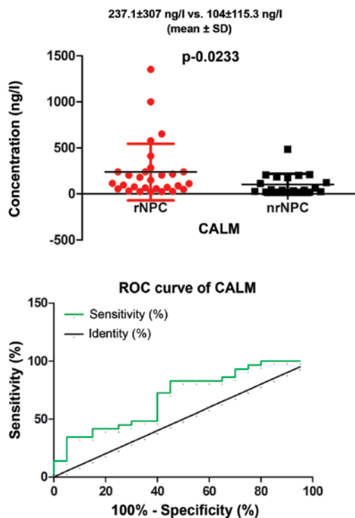
Figure 9. ROC curve of CALM proteins, the area of CALM is 0.6931, P=0.02275 , which showed CALM got some power in clinical used. Compared to nrNPC, the concentration of CALM was higher in rNPC significantly. CALM, calmodulinin; nrNPC, no recurrence nasopharyngeal carcinoma; rNPC, recurrent nasopharyngeal carcinoma.
