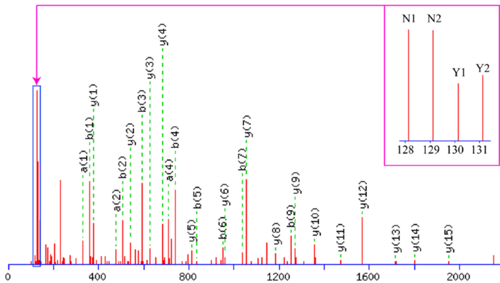
Figure 6. MS/MS spectrum of CALM. MS/MS, tandem mass spectrometry; CALM, calmodulin.
