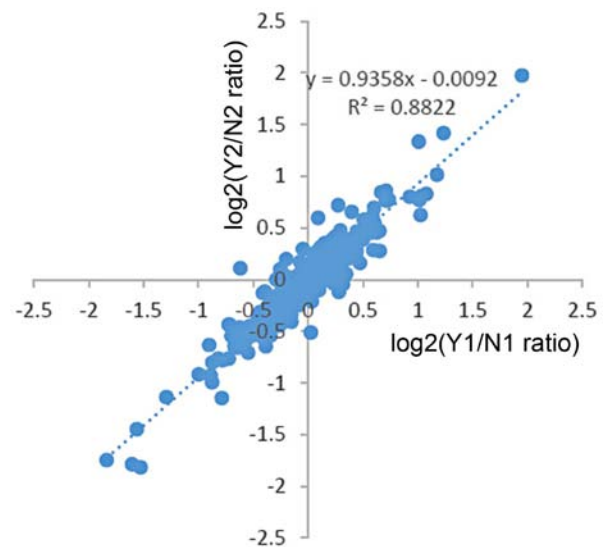
Figure 10. Reproducibility analysis of 2 repeated trials by scatter diagram. The x-axis presents the \log_2(Y1/N1) ratio value and the y-axis presents the \log_2(Y2/N2) ratio value. Y represents recurrent nasopharyngeal carcinoma (rNPC); N represents non-recurrent nasopharyngeal carcinoma (nrNPC).
