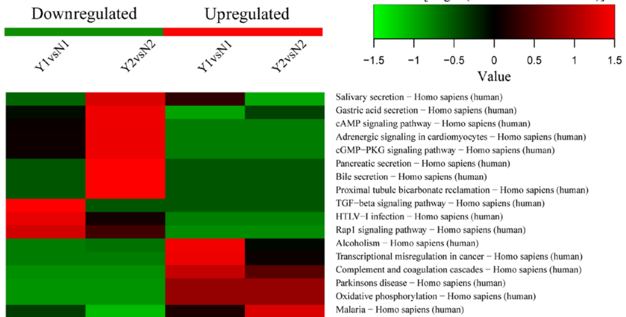
Figure 7. Heatmaps obtained from KEGG enrichment-based cluster analysis, which shown pathway of alcoholism - Homo sapiens (human), salivary secretion - Homo sapiens (human), malaria - Homo sapiens (human), Parkinson's disease - Homo sapiens (human), oxidative phosphorylation - Homo sapiens (human) were meaningful pathways in this process. KEGG, Kyoto Encyclopedia of Genes and Genomes. Y represents recurrent nasopharyngeal carcinoma (rNPC); N represents non-recurrent nasopharyngeal carcinoma (nrNPC).
