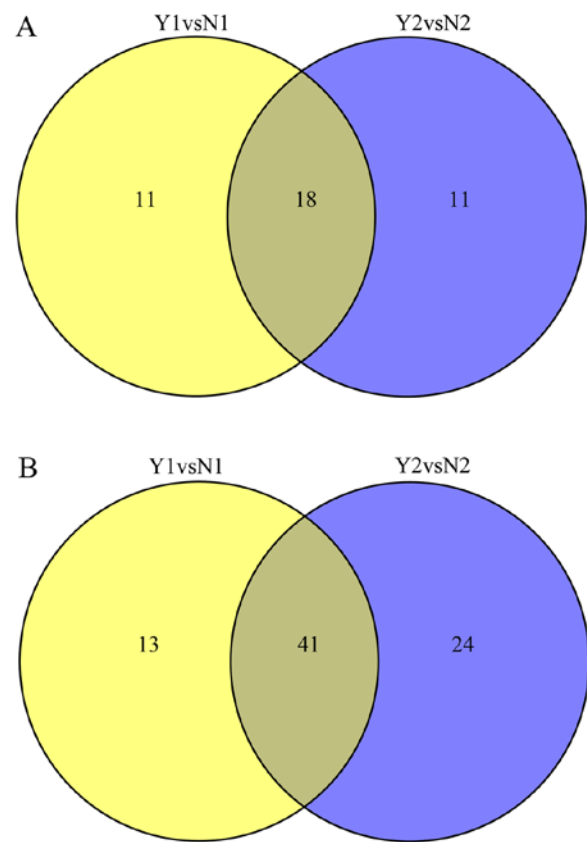
Figure 4. Venn diagrams showing the number of (A) upregulated and (B) down-regulated protein identifications and identification overlap3 of study 1 and 2. Y represents recurrent nasopharyngeal carcinoma (rNPC); N represents non-recurrent nasopharyngeal carcinoma (nrNPC).
