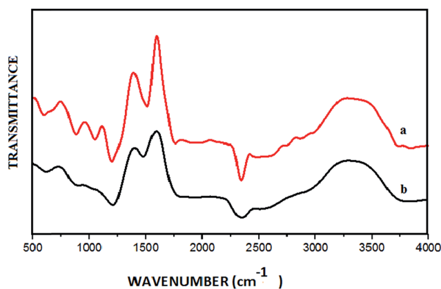
Fig. 3 FT-IR spectra of (a) GO and (b) the CuO NPs/rGO composite.
