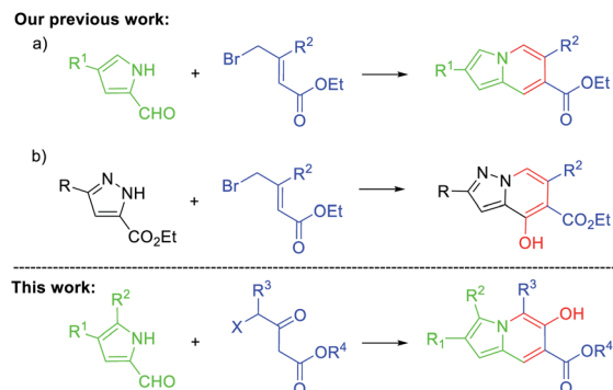
Scheme 1 Access to indolizines via a cascade reaction.
