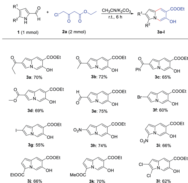
Scheme 2 Substrate scope of pyrrole-2-formaldehyde. Reaction conditions: 1 (1 mmol), 2 (2 mmol), K 2 CO 3 (3 mmol), CH 3 CN (10 mL), 20 °C, 6 h.
