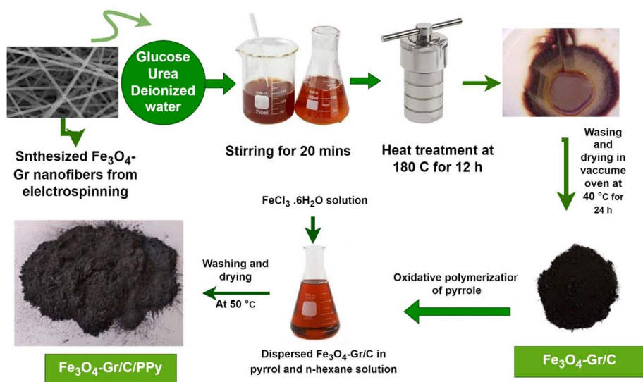
Fig. 1 Pictorial representation of synthesis processes of Fe 3 O 4 -Gr/C/PPy nanofibers composite.
