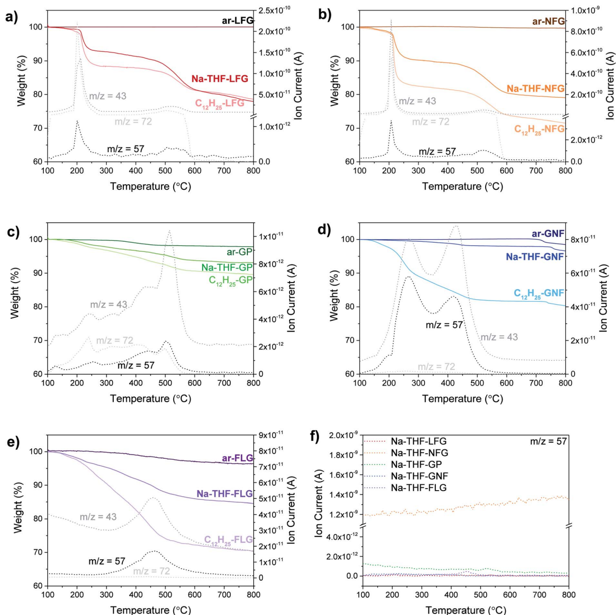
Fig. 2 TGA-MS profiles of ar-, Na-THF, and C_{12}H_{25} - (a) LFG, (b) NFG, (c) GP, (d) GNF and (e) FLG; dodecyl and THF fragments m/z 57 ( C_4H_9^+ ), 43 ( C_3H_7^+/\text{CH}_2\text{O}^- ), 72 ( C_4H_8O ); (f) m/z 57 for each Na-THF-(graphite).
