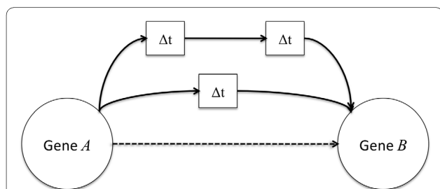
Figure 1 TimeDelay-ARACNE pairwise time MI idea. The basic idea of TimeDelay-ARACNE is to represent the time-shifting in the connections rather than unrolling the activation of nodes in time.
