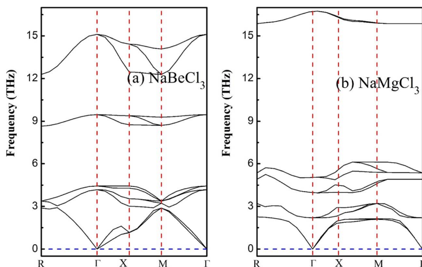
Fig. 8 Phonon dispersion profiles within the irreducible Brillouin zone for the unit cell NaXCl 3 (X = Be, Mg), zone.
