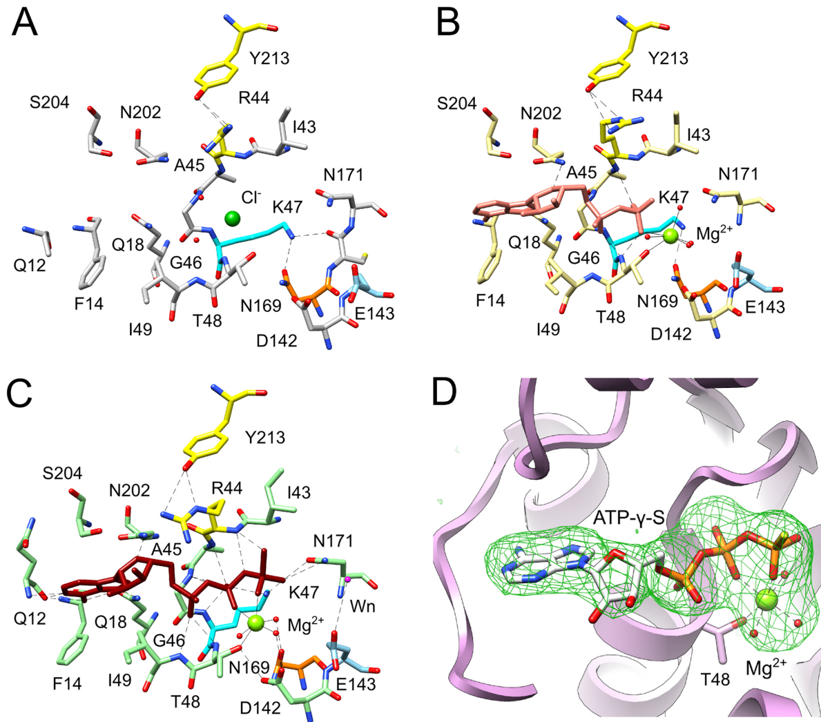
Figure 2. The ATPase active site. The active sites in the structures of (A) apo (grey carbons), (B) ADP complex (khaki carbons) and (C) ATP- \gamma -S complex (green carbons) are shown in ball and stick representation. The P-loop arginine R44 and the lid subdomain Y213 are highlighted in yellow, the P-loop lysine K47 in cyan and the N169 in orange. The catalytic glutamic acid expected to coordinate the catalytic water nucleophile is in blue. (D). The omit electron density map of the ATP- \gamma -S complex, contoured at 3\sigma level, was calculated after omitting ATP- \gamma -S and the coordinated metal from the model. Hydrogen bonding interactions on all diagrams are in black dashed lines, coordination to the metal ( Mg^{2+} , green sphere) is shown by a continuous black line.
