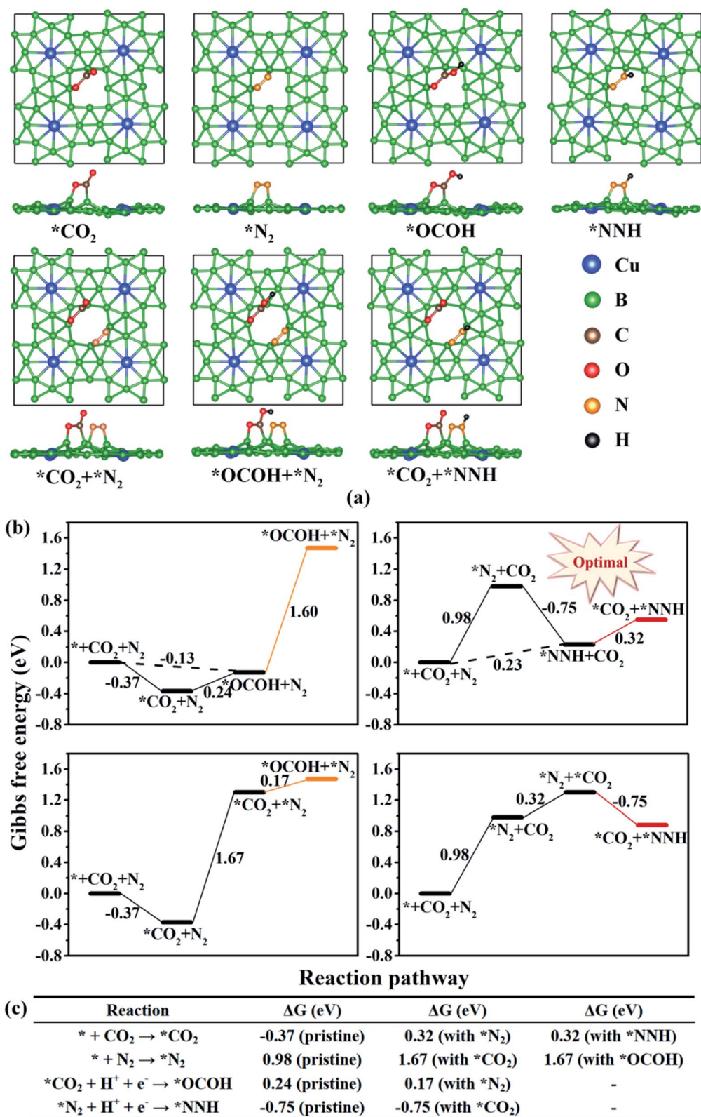
Fig. 3 (a) Top and side views of the optimal geometric structures for *\text{CO}_2 , *\text{N}_2 , *\text{OCOH} , *\text{NNH} , *\text{CO}_2 + *\text{N}_2 , *\text{OCOH} + *\text{N}_2 and *\text{CO}_2 + *\text{NNH} on the \text{CuB}_{12} monolayer. (b) Gibbs free energy diagrams for the first hydrogenation process of \text{CO}_2 and \text{N}_2 reduced to a *\text{OCOH} + *\text{N}_2 intermediate and *\text{CO}_2 + *\text{NNH} intermediate. (c) Calculated Gibbs free energy change values ( \Delta G , eV) for the four elementary reactions on the pristine \text{CuB}_{12} monolayer and the \text{CuB}_{12} monolayer with other adsorption intermediates.
