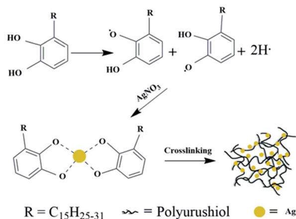
Fig. 1 Schematic in situ fabrication of PUL/AgNPs.
