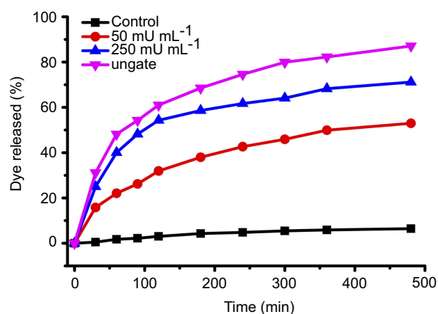
Figure 3 Release profiles of Flu from un gated-MSN or MSN-SC 6 A stimulated by different concentrations of AChE. -■-: Control, MSN-SC 6 A without external stimuli; -●-: MSN-SC 6 A triggered by 50 mU/mL AChE; -▲-: MSN-SC 6 A triggered by 250 mU/mL AChE; -▼-: un gated-MSN (mean ± SD, n=3 for each sample).
