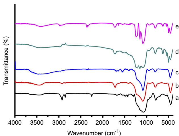
Figure S3 FTIR spectra of MSN-CN (A), MSN-COOH (B), MSN-COOR (C), MSN-Ch (D) and MSN-SC 6 A (E).
