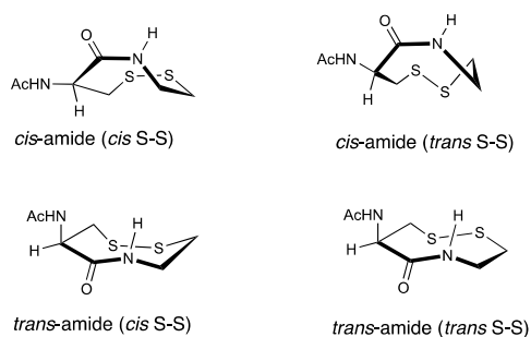
Figure 1. Conformations of \mathbf{1}^{\text{ox}} .
