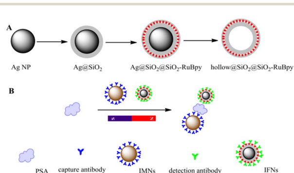
Fig. 9 (A) Schematic illustration for synthesis of Ag@SiO 2 @SiO 2 -RuBpy and hollow@SiO 2 @SiO 2 -RuBpy. (B) Schematic illustration for the construction of the detection of PSA with the immunomagnetic nanospheres and immunofluorescent NPs. Reprinted with permission from ref. 111 Copyright (2017) Elsevier.
