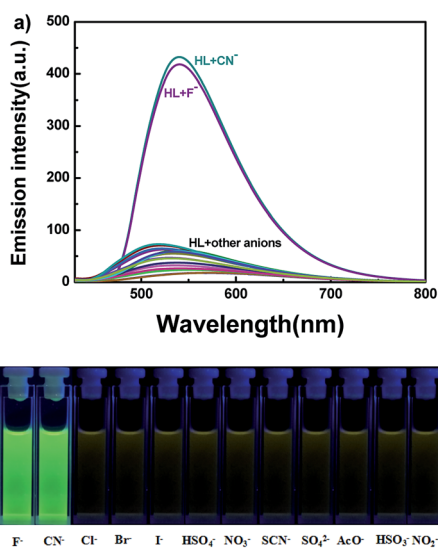
Fig. 7 (a) The change in fluorescence spectra of HL induced by various anions (5.0 equiv.) in acetonitrile ( 2.0 \times 10^{-5} \text{ mol L}^{-1} ) (excited at 420 nm); (b) photos of color changes in acetonitrile.
