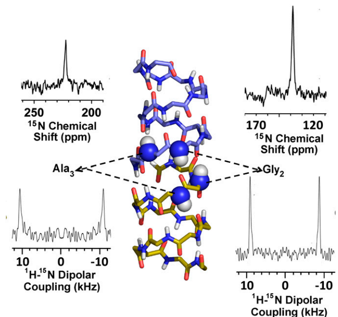
Fig. 1. Slices through the ^1\text{H} - ^{15}\text{N} dipolar and ^{15}\text{N} anisotropic chemical shift dimensions of the 2D OS ssNMR (SAMPI4) spectra of ^{15}\text{N} G2- and ^{15}\text{N} A3-labeled gA at 35.2 T (36), showing excellent alignment of gA in liquid-crystalline lipid bilayers of DMPC and precise dimeric symmetry of the structure. The gramicidin structure is a dimer (upper monomer carbon is light blue and nitrogen dark blue; lower monomer carbon is gold and nitrogen dark blue). Oxygen is red and hydrogen is white. This illustrates the two ^{15}\text{N} - ^1\text{H} sites in each subunit (dark blue and white spheres) that were ^{15}\text{N} -labeled for this OS ssNMR sample in the liquid-crystalline preparation. The spectrum of the two A3 sites is shown on the left and the two G2 sites on the right.
