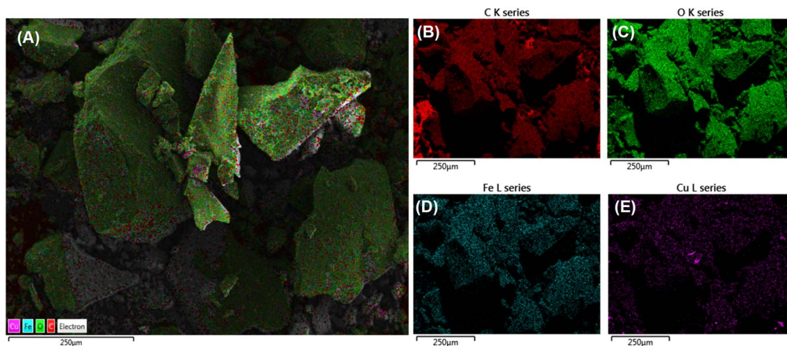
Fig. 4 The EDS layered image (A), EDS element mapping images of C (B), O (C), Fe (D) and Cu (E) for Fe–Cu-BTC sample.
