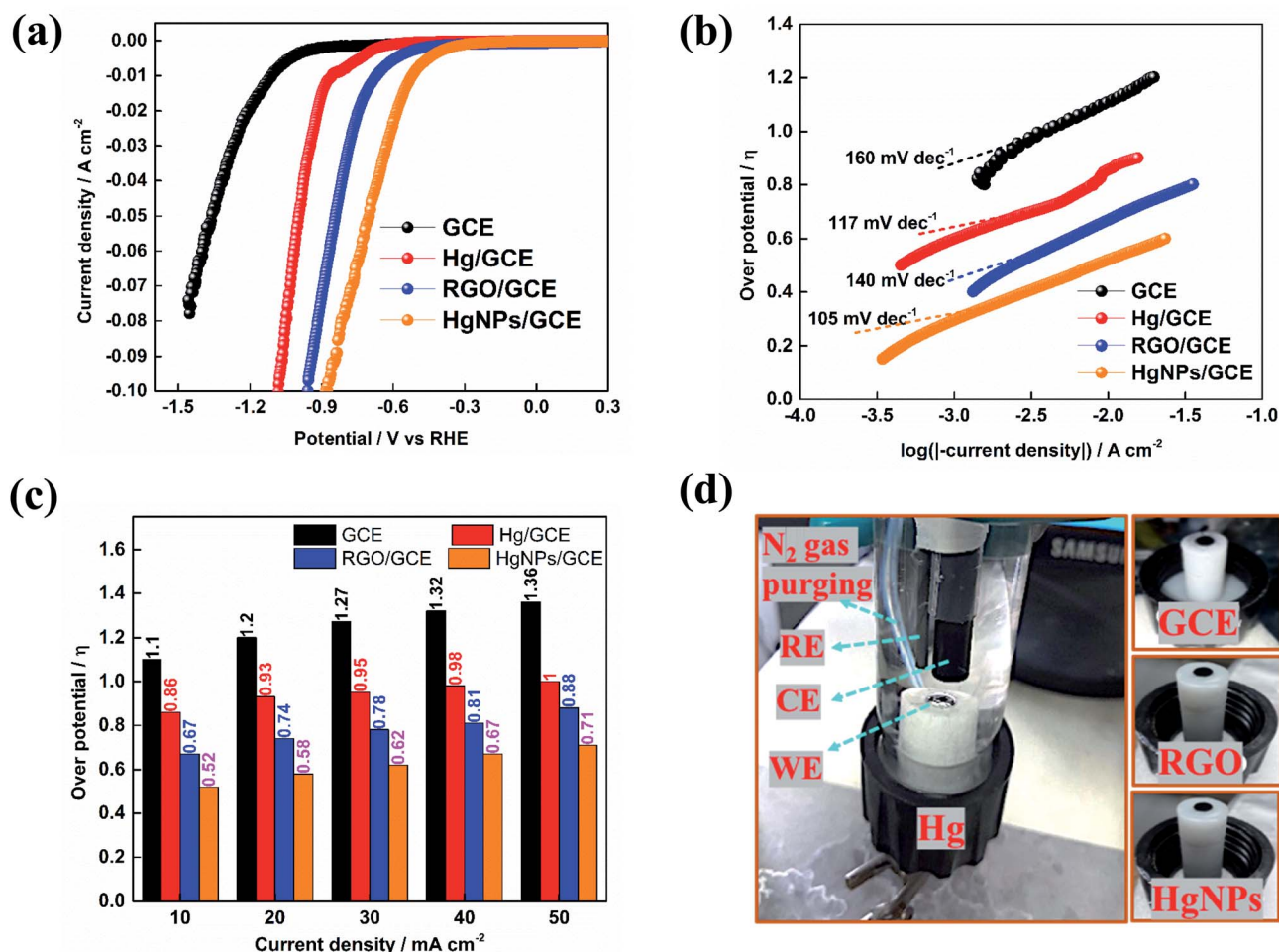
Fig. 5 Results of HER study by linear sweep voltammetry using GC, Hg/GC, RGO/GC and HgNPs/GC electrodes in 0.5 M H 2 SO 4 solution at 10 mV s -1 . (a) Potentio-dynamic behavior of HER with the four electrodes (b) Tafel plots, (c) histograms comparing the onset overpotential and (d) photograph of the electrochemical cell configuration for HER study.
